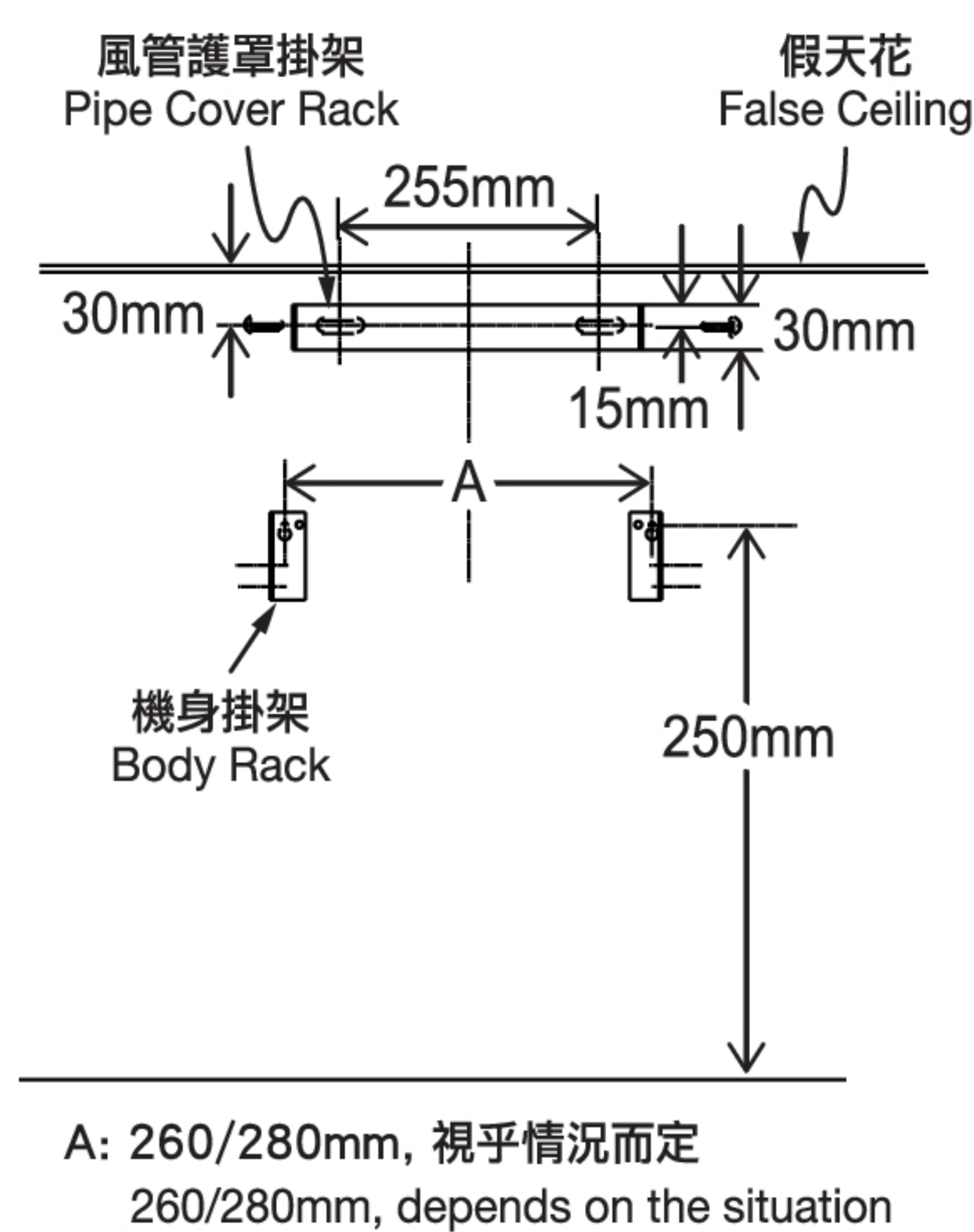
掛牆螺絲孔位置 Screw Position on Wall
