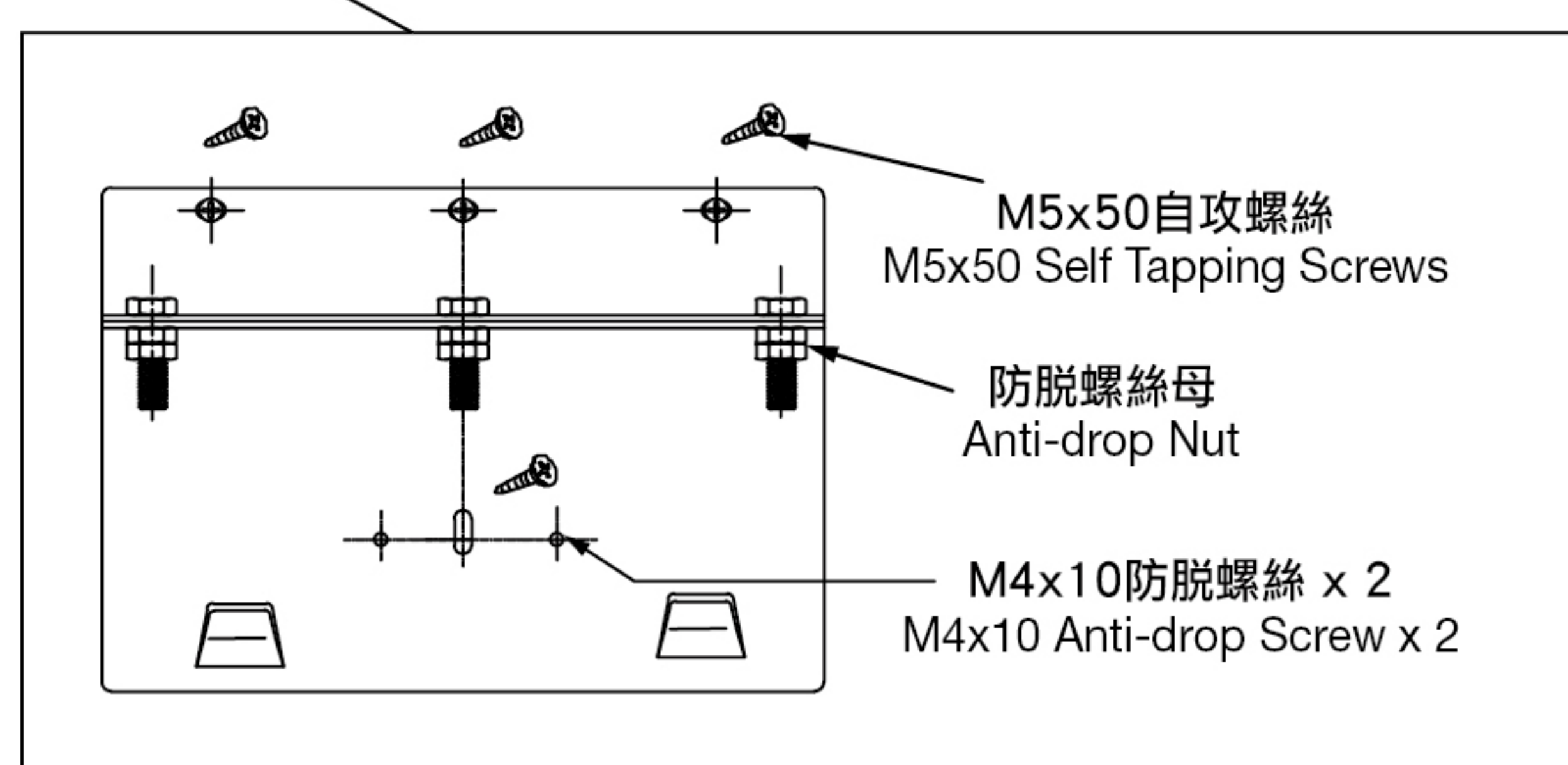
掛牆螺絲孔位置 Screw Position on Wall
