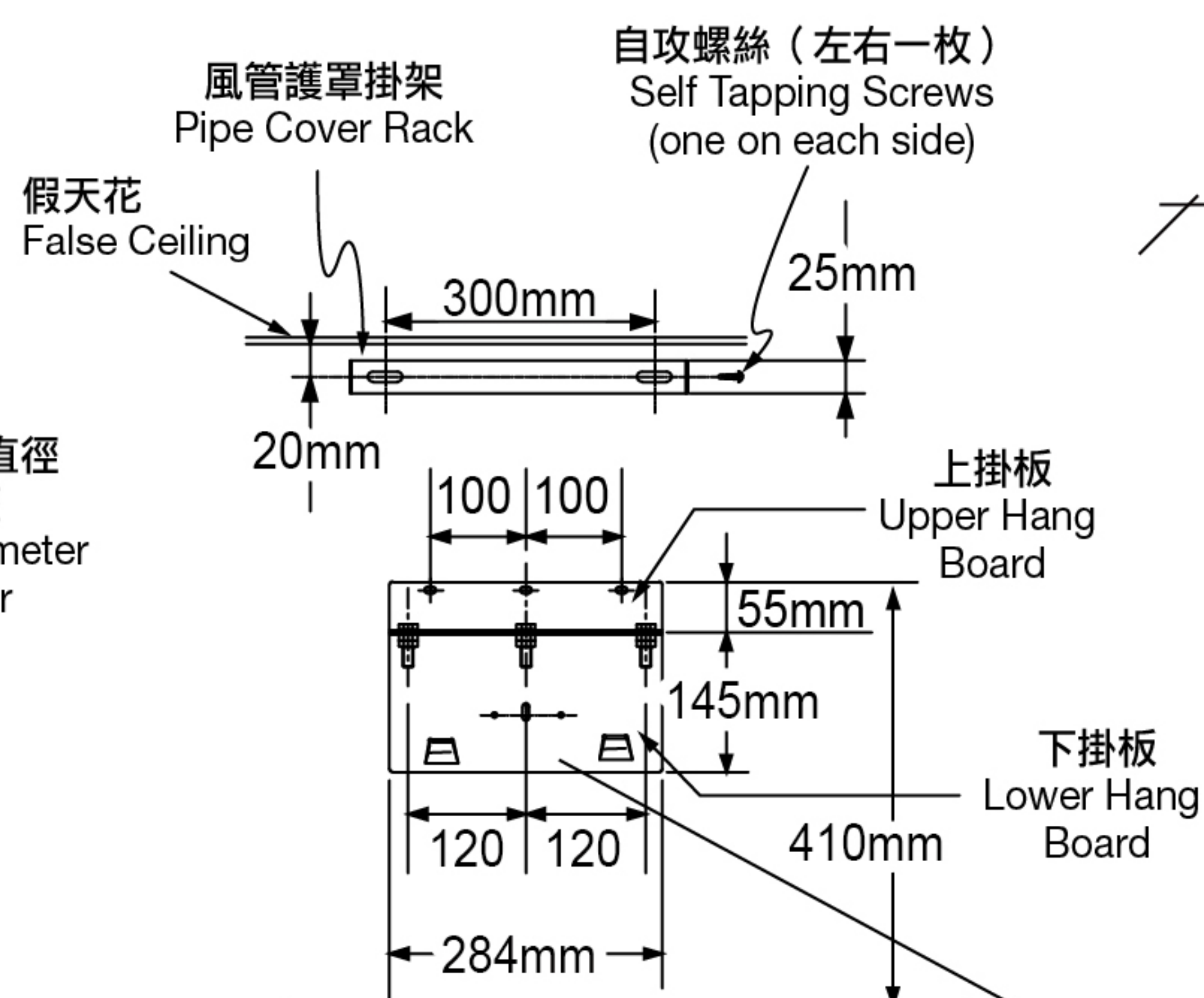
掛牆螺絲孔位置 Screw Position on Wall
