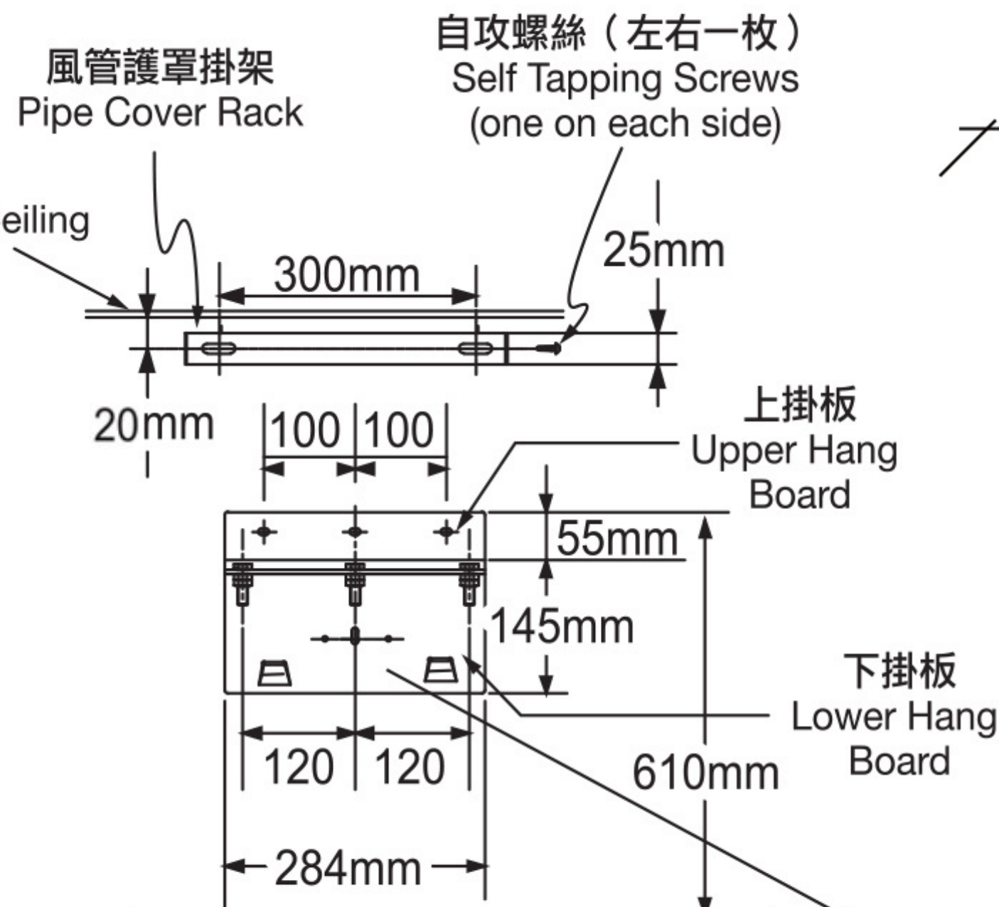
掛牆螺絲孔位置 Screw Position on Wall
