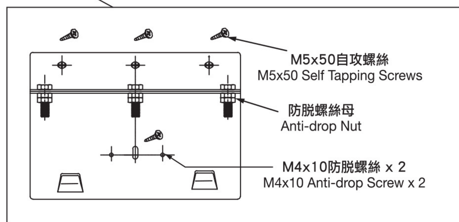
掛牆螺絲孔位置 Screw Position on Wall
