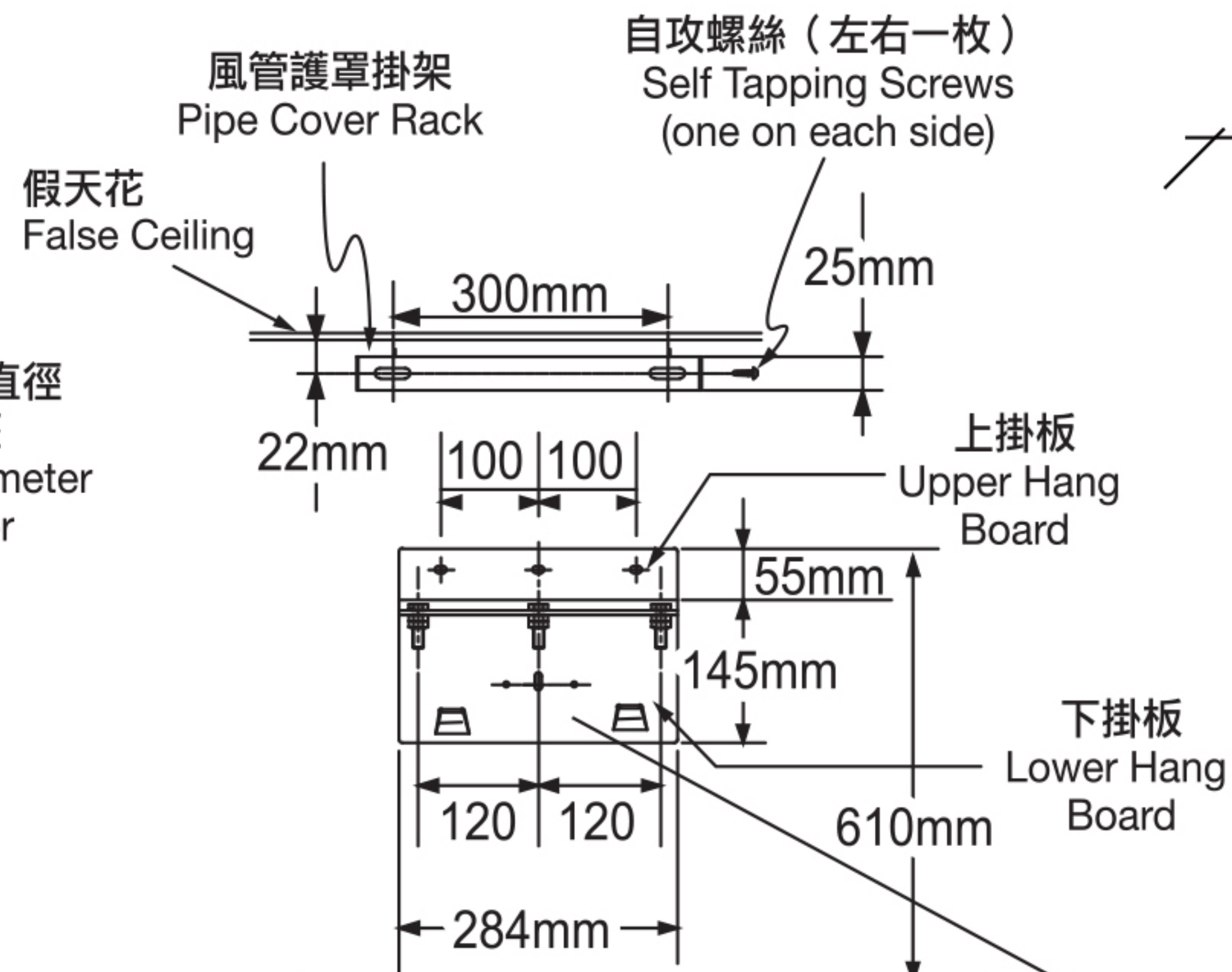
掛牆螺絲孔位置 Screw Position on Wall
