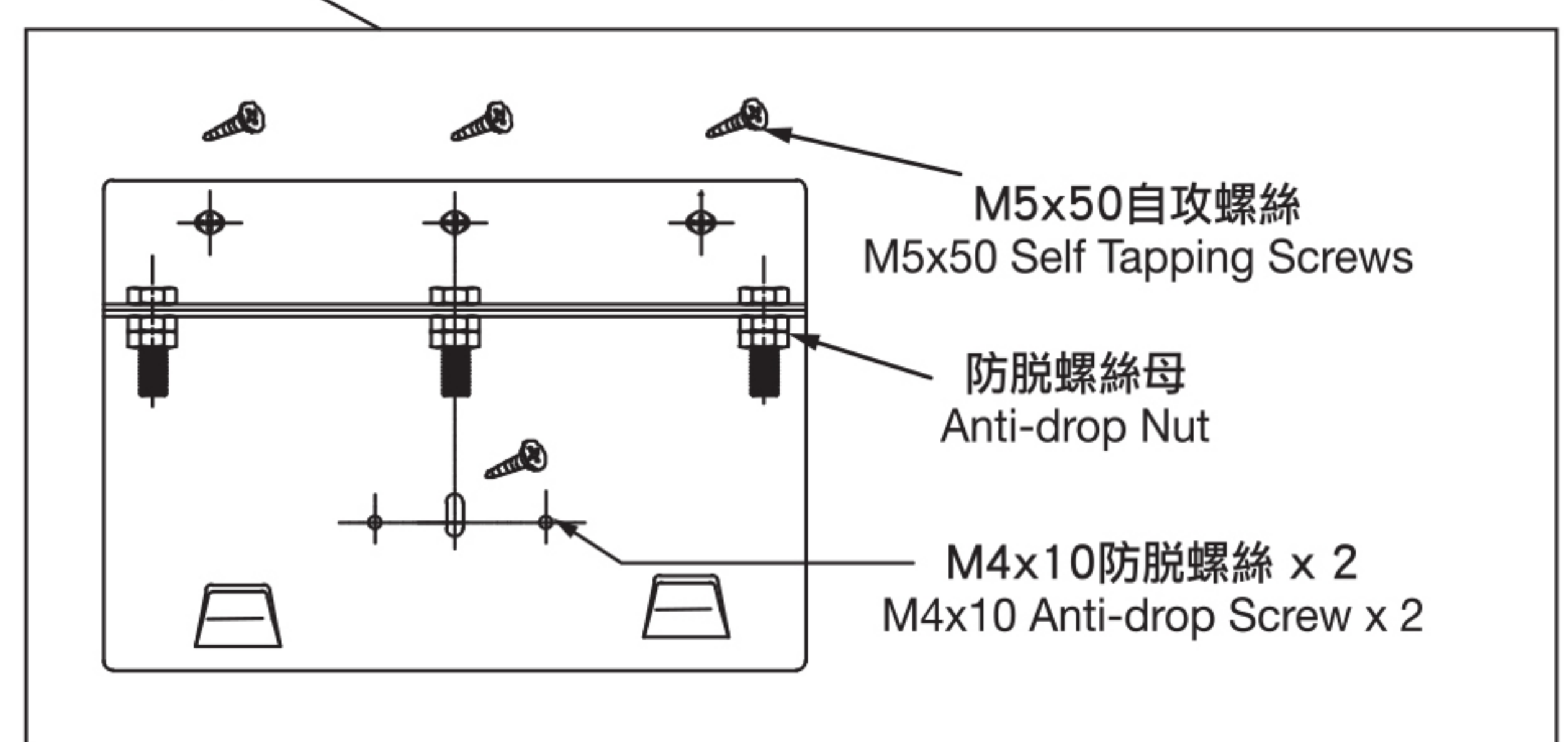
掛牆螺絲孔位置 Screw Position on Wall
