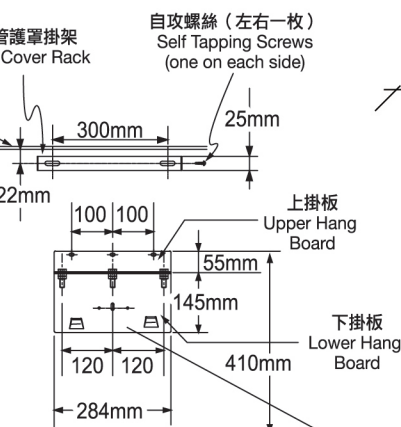
掛牆螺絲孔位置 Screw Position on Wall
