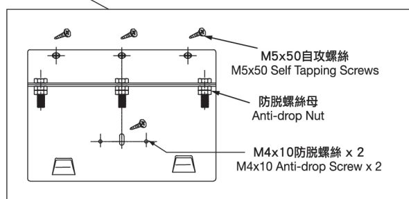
掛牆螺絲孔位置 Screw Position on Wall
