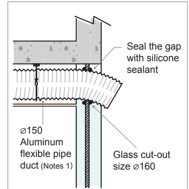
Exhaust outlet on the glass
