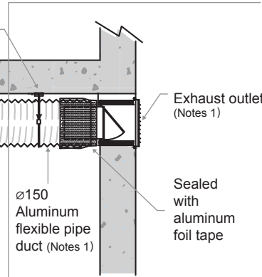
Exhaust outlet on the wall
